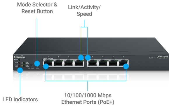
EWS2908P
